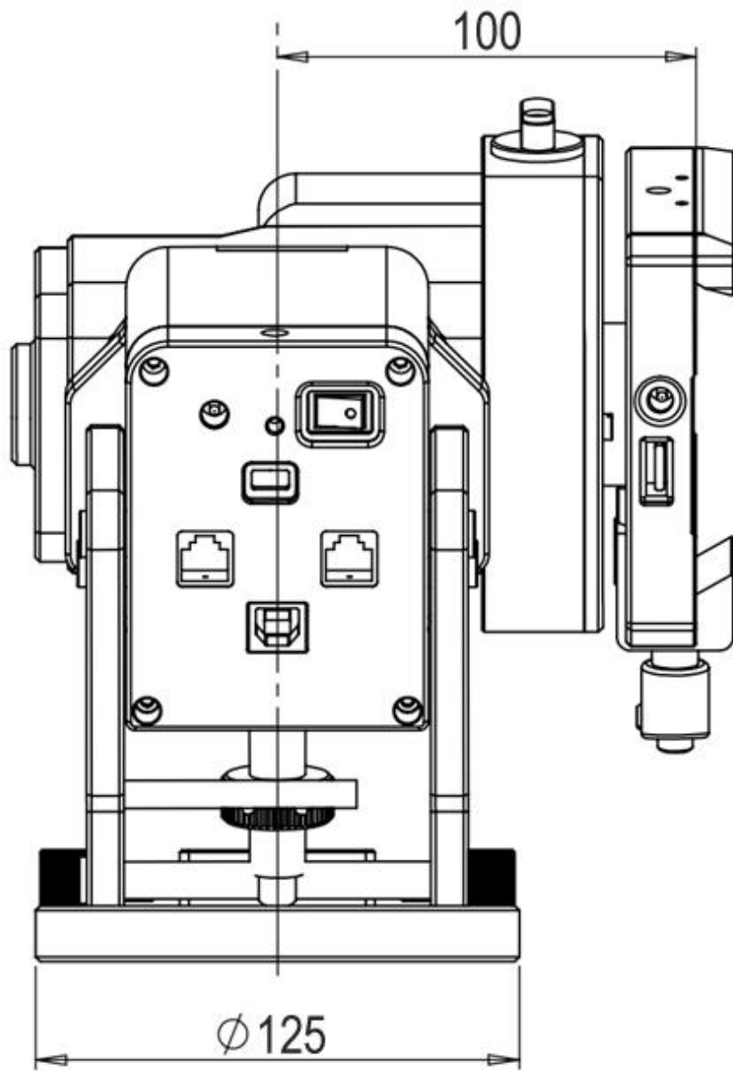
Figure 23 Distance between HEM44 RA axis and base of dovetail saddle
