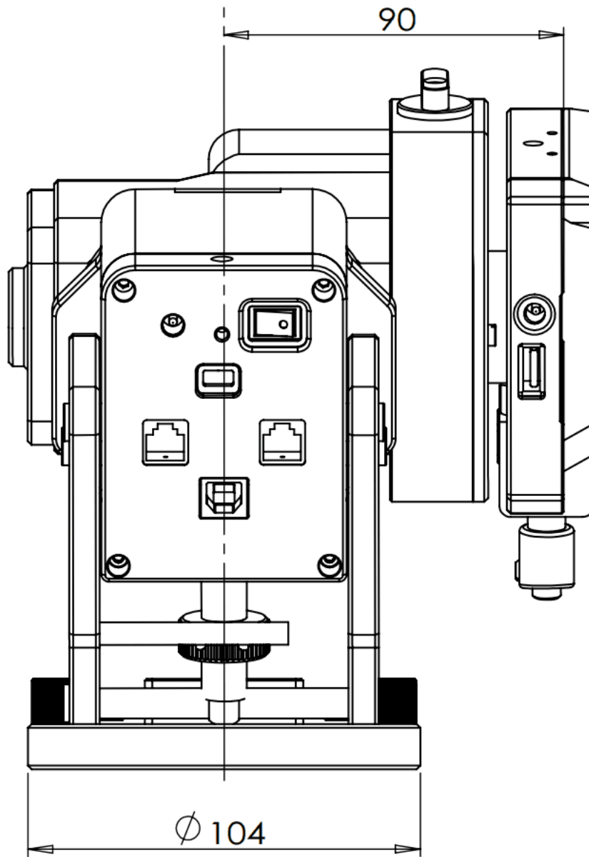
Figure 24 Distance between HEM RA axis and base of dovetail saddle
