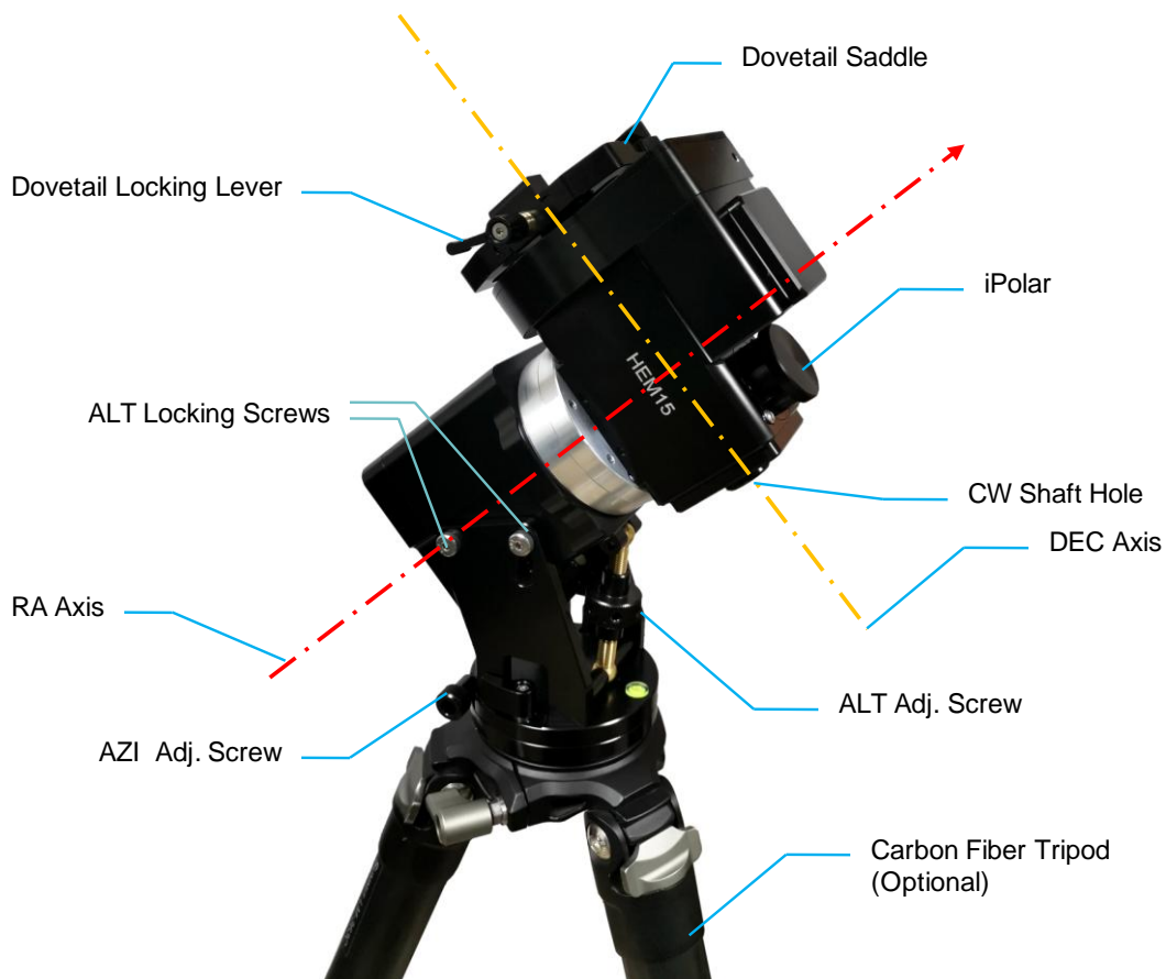
Figure 1. HEM15 mount assembly
