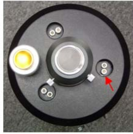
Figure 6b. Now, turn the push screw in the same set clockwise no more than \frac{1}{4} turn.
