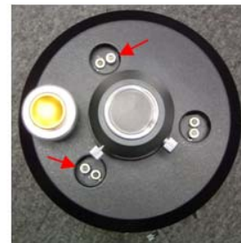
Figure 7d. Turn the two push screws in these two sets clockwise no more than \frac{1}{4} turn.
