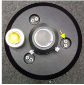
Figure 6a. Turn the pull screw counterclockwise a small amount, no more than a \frac{1}{4} turn. (Note: actual selected alignment screw will vary.)
