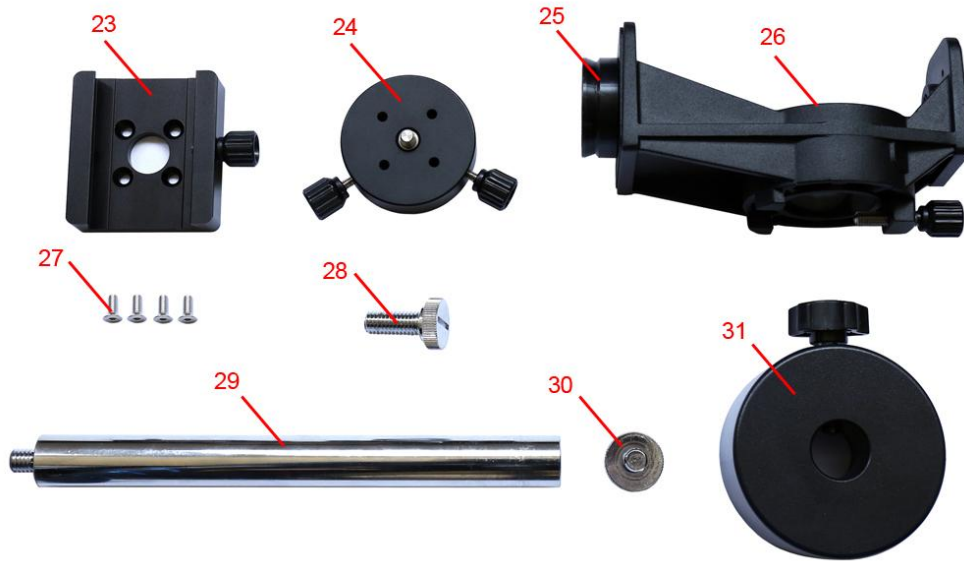
Figure 7. DEC mounting bracket and counterweight package
